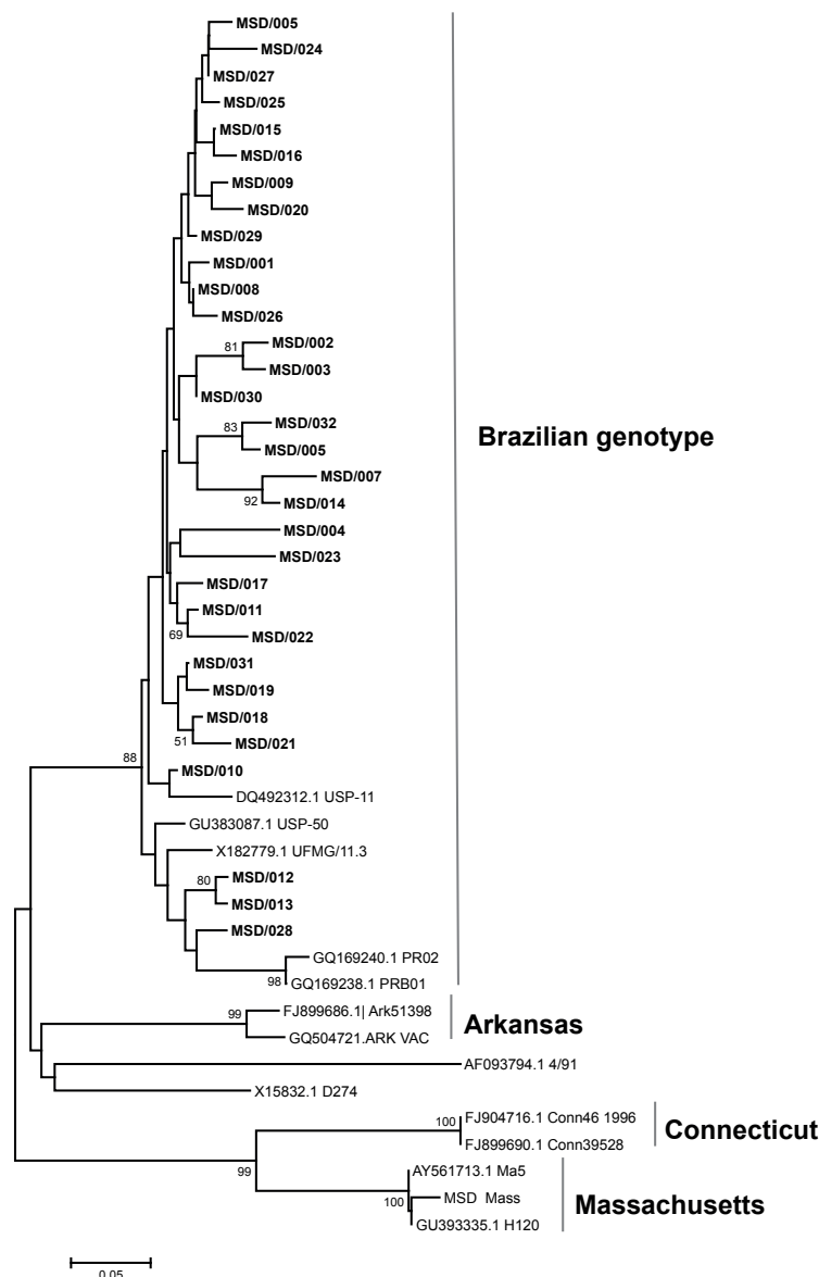
Fig. 1 Amino-acid neighbour-joining maximum composite, likelihood (NJ MCL) tree for the partial sequences of the S1 subunit of the avian infectious bronchitis virus spike gene
