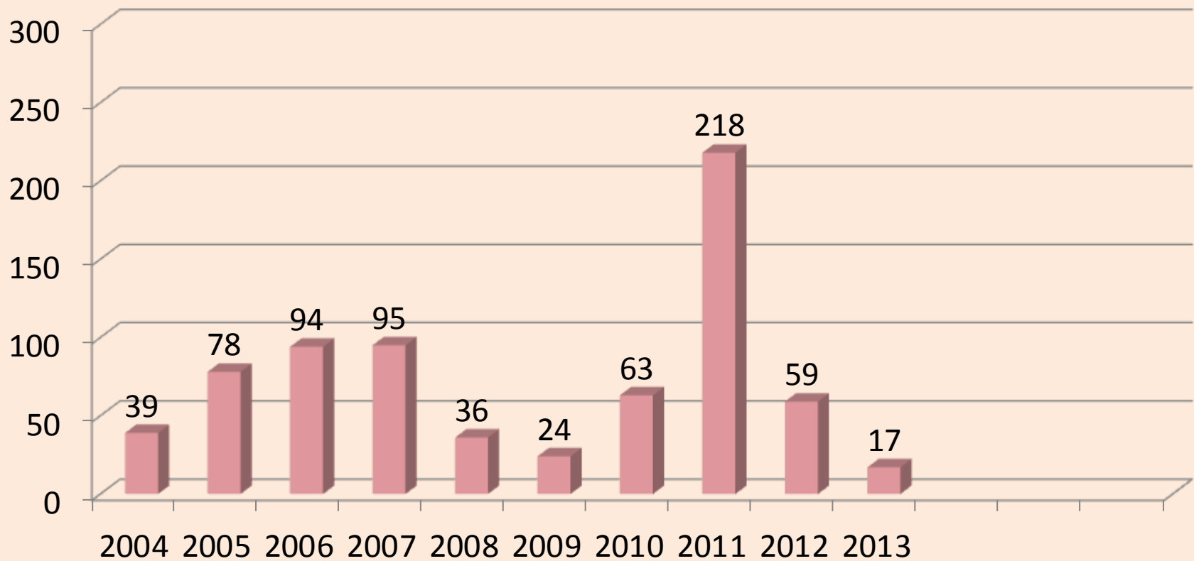
PPR Outbreaks & Years 2004-2013 up to September
